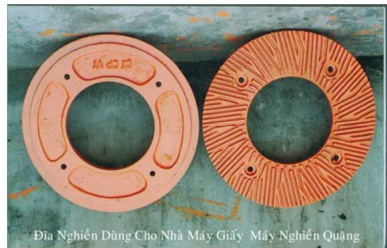
Grind disc for paper and ore crusher
